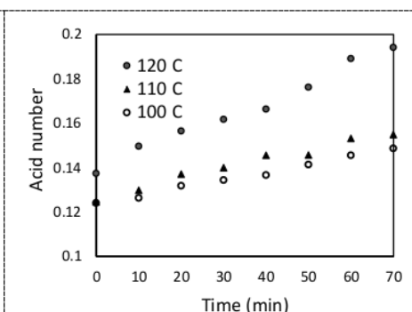
Figure 2. Acid numbers of the mixture of biodiesel B20 and soursop leaf extract antioxidant during the oxidation process with air (operating conditions: rotation speed of 600 rpm and air velocity of 2.3 L/min).
