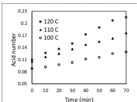
Figure 1. Acid numbers of biodiesel B20 during the oxidation process with air (operating conditions: rotation speed of 600 rpm and air velocity of 2.3 L/min).
