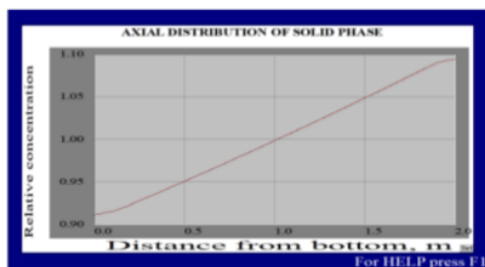
Figure 6. Axial distribution of solid phase in equal blend time parameter.
