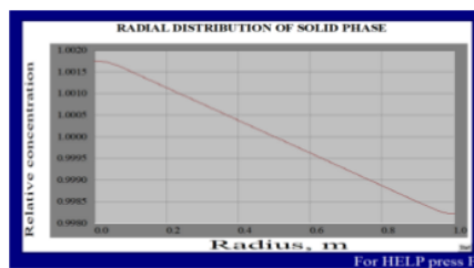
Figure 7. Radial distribution of solid phase in equal blend time.
