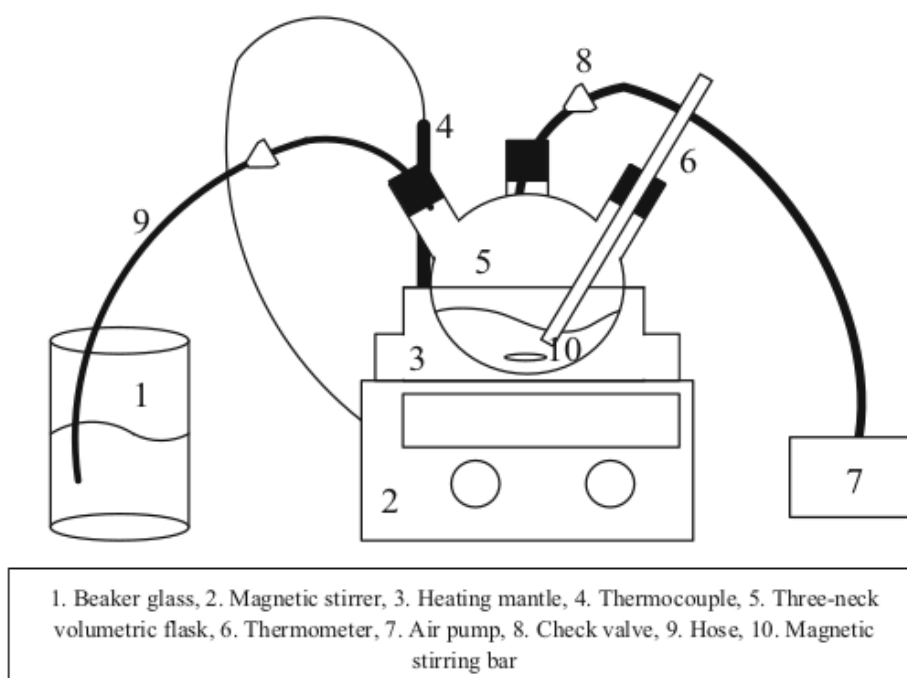
Fig. 2.10 Equipment of biodiesel oxidation with air
