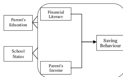
Figure 1. Theoretical Framework
