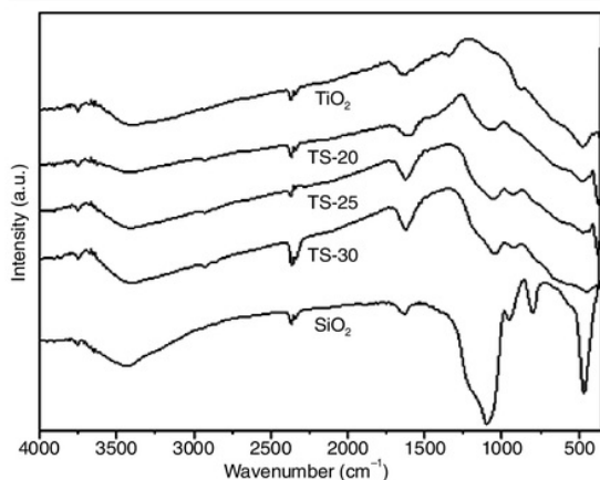
Fig. 2. FT-IR spectra for Titania-Silica-PVA nanocomposites
