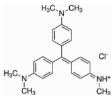
Gambar 1. Struktur molekul methyl violet
