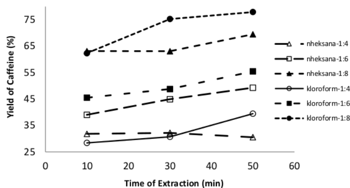
Figure 3. Effect of solvent variation, volume ratio, and extraction time on the caffeine extraction from coffee shell bio-oil.
