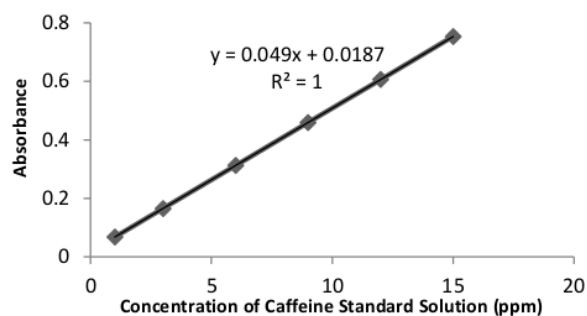
Figure 2. Calibration curve of standard caffeine solution.
