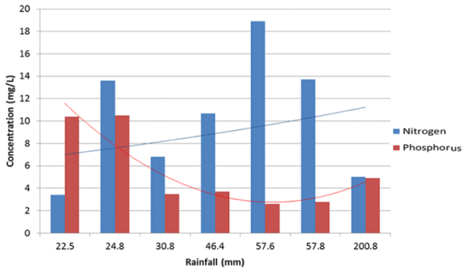
Fig. 3: The correlation between rainfall and nutrient loss on vineyard area in Penedes, Spain.
