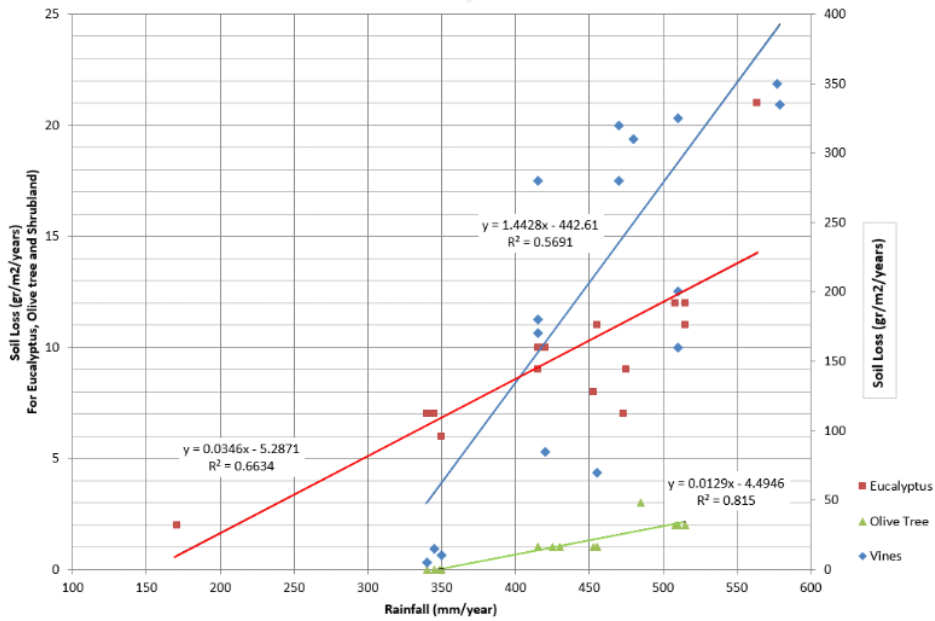
Fig. 1: The correlation between rainfall and soil loss from three different types of vegetation.
