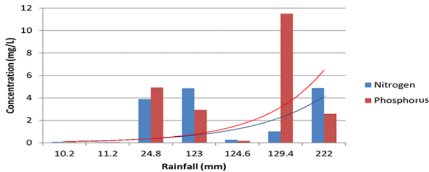
Fig. 4: The correlation between rainfall and nutrient loss on vineyard area.
