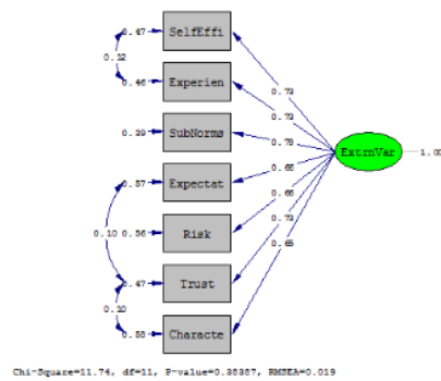
Figure 2. Output Standardized Solution Model of External Variables Figure 3. Output T-Values Model of External Variables
