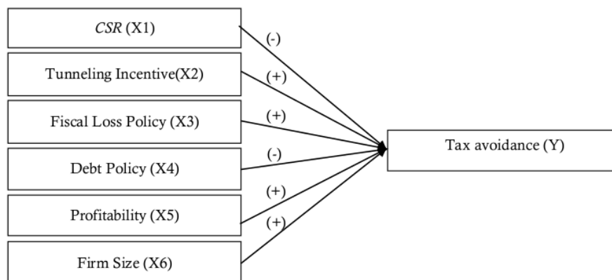
Figure 1. Theoretical Framework
