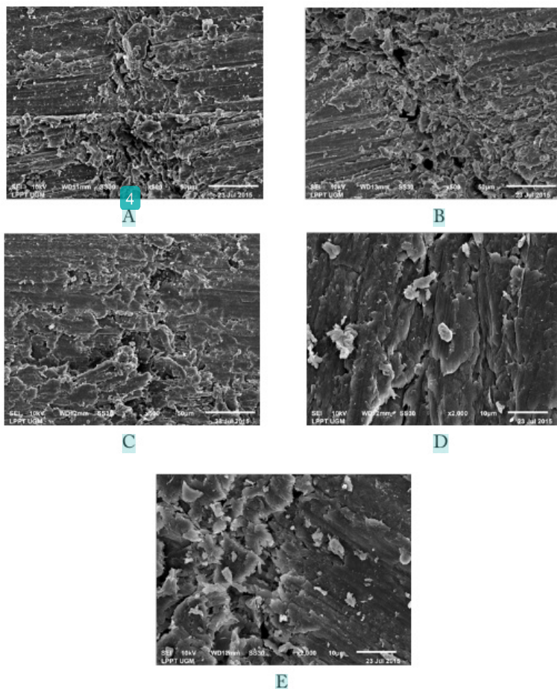
Fig. 2: Scanning electron micrograph of the transverse section of five bamboo fiberboard after termites' attack: (A) Dendrocalamus asper ; (B) Bambusa vulgaris ; (C) Gigantochloa atroviolacea ; (D) Gigantochloa apus ; (E) Gigantochloa atter .
