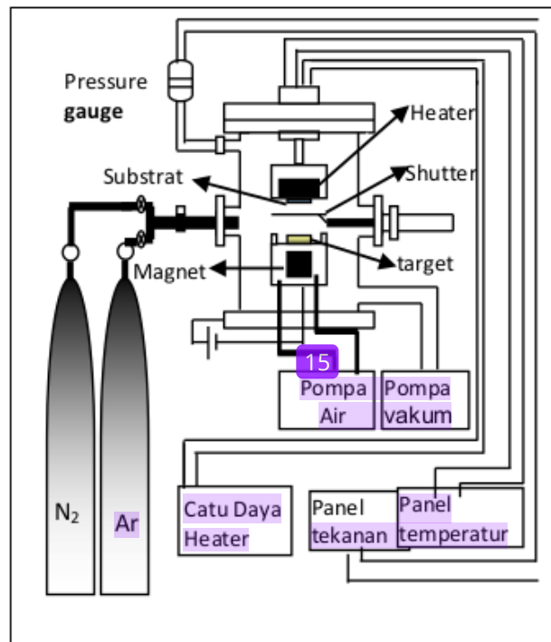
Gambar 3.2 Skema reaktor DC magnetron sputtering
