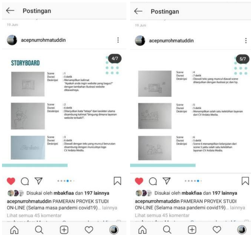
Gambar 3 Storyboard scene 1-6
