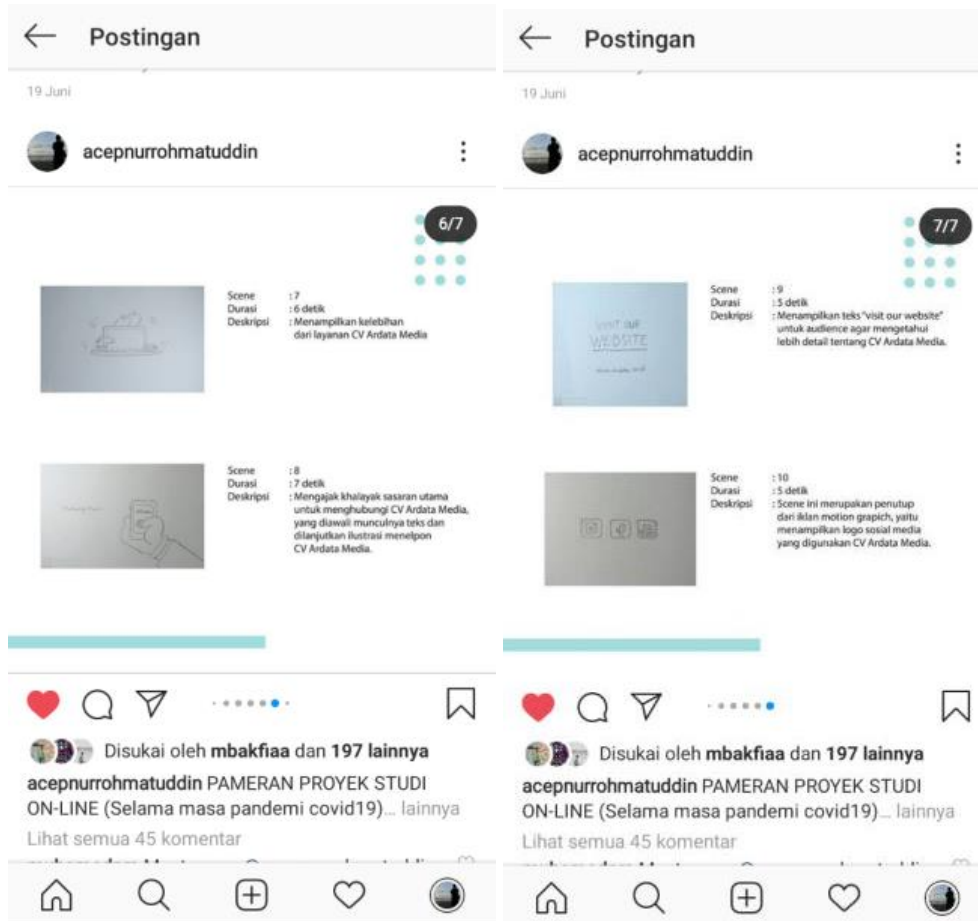
Gambar 4 Storyboard scene 7-10
