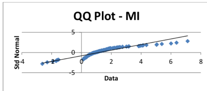
FIGURE 2. QQ Plot-MI
