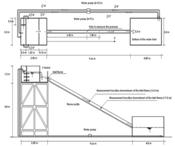
Figure 2 The layout of device and instruments of the study
