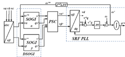
Figure 4. Block diagram of DSOGI PLL
