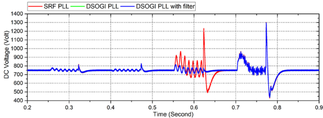
Figure 9. DC voltage condition in several cases using DSOGI PLL with filter, DSOGI PLL, and SRF PLL under several conditions.
