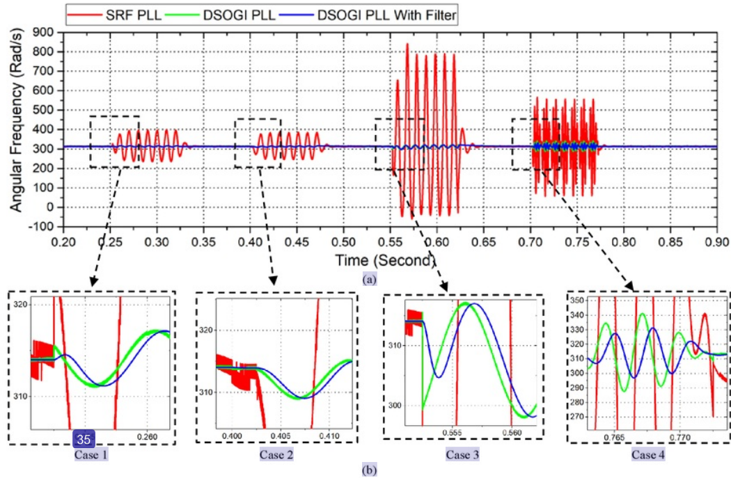
Figure 8. Frequency estimation (a) frequency estimation of DSOGI PLL with filter, DSOGI PLL, and SRF PLL under several conditions (b) performance frequency estimation of DSOGI PLL with filter under several conditions.
