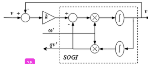
Figure 3. Block diagram of a Second Order Generalized Integrator.
