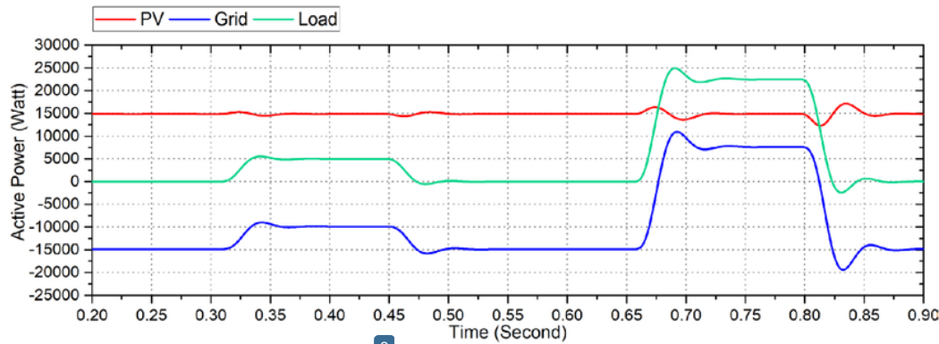
Figure 13. Power flow condition under linear and non-linear load using DSOGI PLL with filter.
