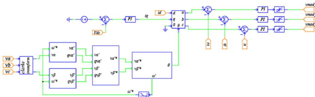
Figure 6. Simulink model of synchronization, current control, and DC link control.
