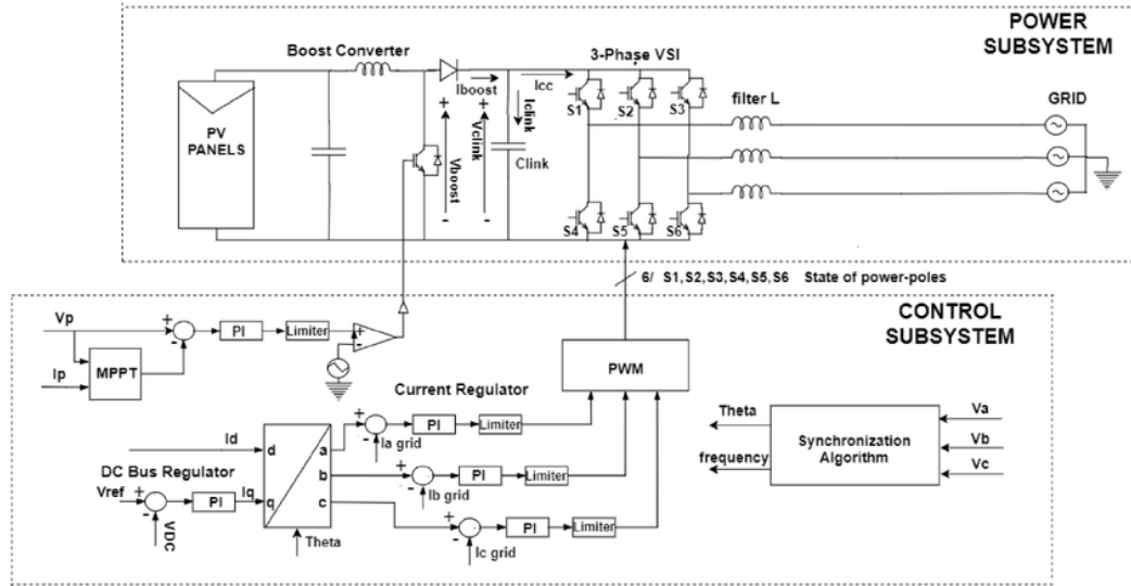
Figure 1. Block diagram of three-phase grid-connected photovoltaic system.
