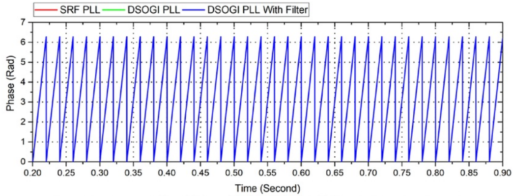
Figure 10. Phase estimation of DSOGI PLL with filter, DSOGI PLL, and SRF PLL under linear and non-linear load.
