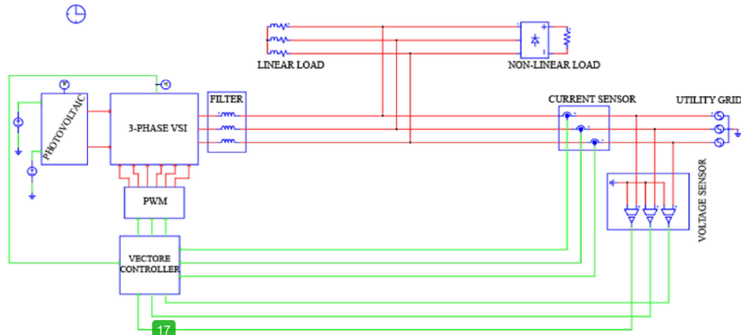
Figure 5. Simulink model of three-phase grid-connected photovoltaic system on PSIM.
