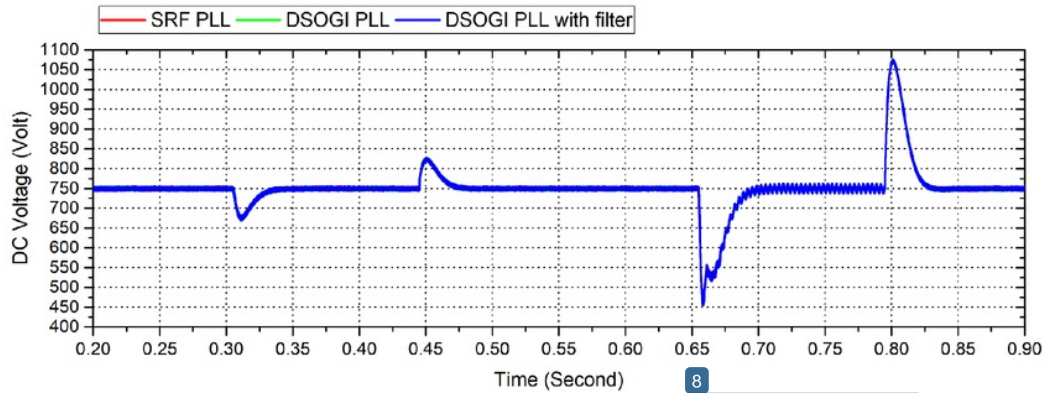
Figure 12. DC voltage of DSOGI PLL with filter, DSOGI PLL, and SRF PLL under linear and non-linear load.
