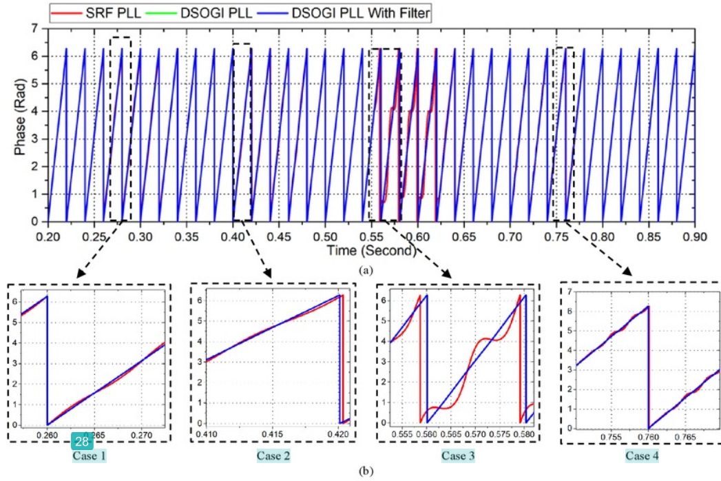
Figure 7. Phase estimation (a) phase estimation of DSOGI PLL with filter, DSOGI PLL, and SRF PLL under several conditions (b) performance phase estimation of DSOGI PLL with filter under several conditions.
