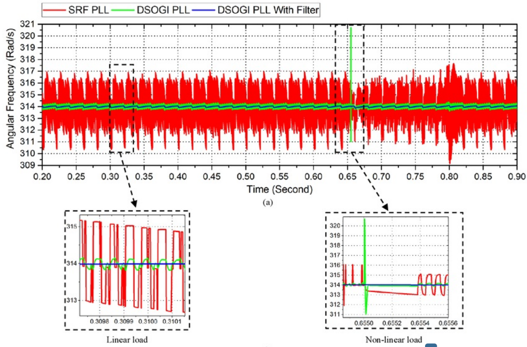
Figure 11. Frequency estimation (a) frequency estimation of DSOGI PLL with filter, DSOGI PLL, and SRF PLL under linear and non-linear load.
