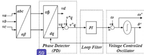
Figure 2. Block diagram of SRF PLL for Three Phase
