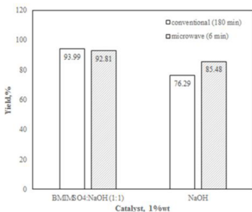
Figure 5. Effect of microwave and conventional heating in the transesterification reaction of the biodiesel yield
