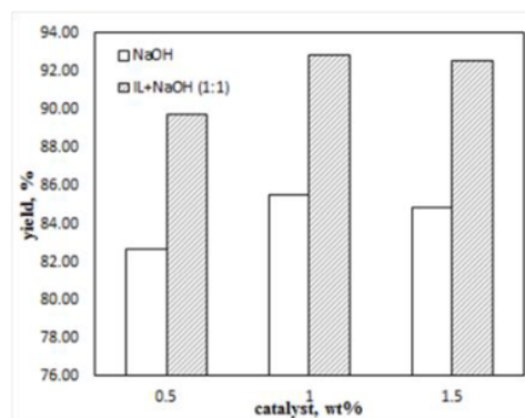
Figure 2. The effect of catalyst concentration to biodiesel yield during the microwave assisted esterification. The catalyst was compared between homogenous catalyst (NaOH) and a mixed catalyst (Ionic Liquid and NaOH at 1:1 vol. ratio) in the range of 0.5-1.5 % (w/w)
