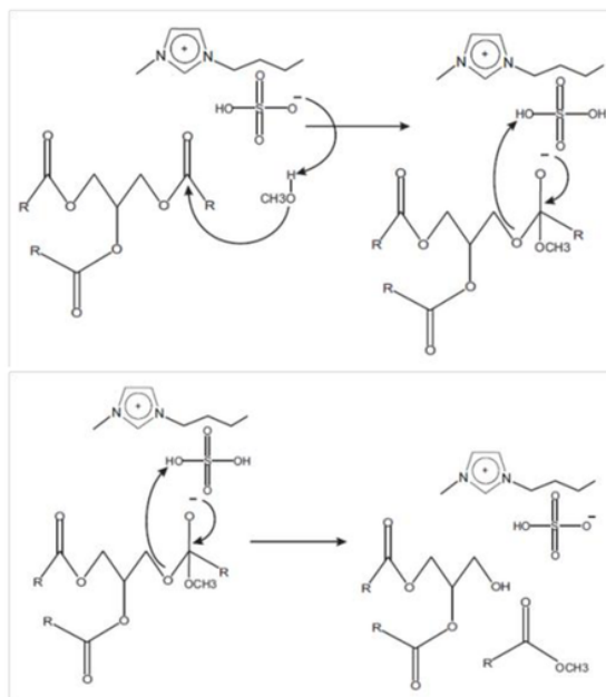
Figure 4. The reaction mechanism of triglyceride and methanol using the ionic liquid [BMIMHSO 4 ] as catalyst [11]
