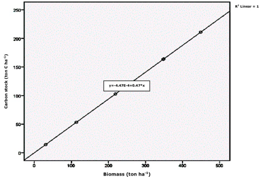
Figure 3. Correlation graph of biomass and carbon stock (Source: Data analysis, 2016).
