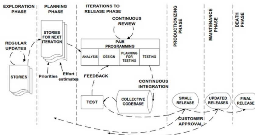
Figure 4. Process of Extreme Programming
