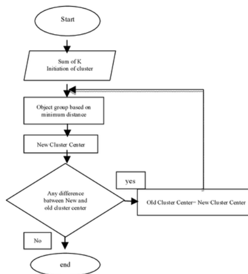
Figure 1. K-Means Algorithm
