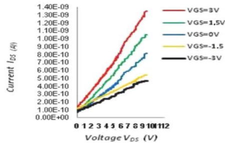
Figure 5. Characteristics OFET with channel length of 100 \mu\text{m} .
