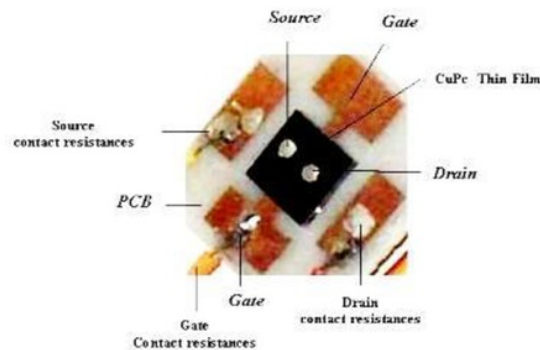
Figure 4. Results OFET fabrication on PCB
