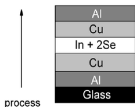
Figure 1. Elemental Stacking Order of the Precursors
