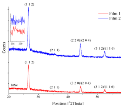
Figure 4. X-ray Diffraction Patterns of film 1 and 2
